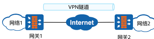
Site-to-Site VPN
